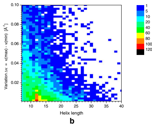
Fig. 4 Variation of the curvature \Delta\kappa = \kappa(max) - \kappa(min) in \text{\AA}^{-1} of protein helices depending on helix length (i.e., number of residues) given (a) as general distribution in form of a 3D bar diagram (color is used to distinguish between helices of length m and m+1 ) and (b) in a detailed 2D distribution diagram where the frequencies of \Delta\kappa values for specific helix lengths is color-coded. The curvature of the helix axis is determined after fitting all axis directions with a third-order polynomial. Only helices with seven or more residues are considered
