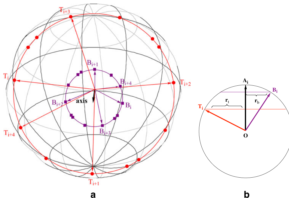
Fig. 2 a If the unit binormal vectors \mathbf{B}_i of all anchor points of a helix are moved to a common origin, O , and the unit tangent vectors \mathbf{T}_i to the same point, their end points lie on two circles on the surface of the circumscribed sphere with unit radius and origin O . b The associated vectors \mathbf{T}_i and \mathbf{B}_i lie on a slice through the sphere where the trace of the sphere is given as a unit circle and the diameters of the surface circles
