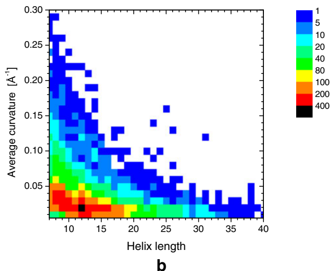
Fig. 3 Average curvature \kappa_{av} in \text{\AA}^{-1} of protein helices as a factor of helix length (i.e., number of residues) given (a) as general distribution in form of a 3D bar diagram (color is used to distinguish between helices of length m and m+1 ) and (b) in a detailed 2D distribution diagram where the frequencies of axis curvatures for specific helix lengths is color-coded. The curvature of the helix axis is determined after fitting all axis directions with a third-order polynomial. Only helices with seven or more residues are considered
