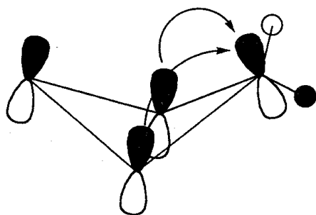
HOMO (allyl) - pseudo- \pi^* ( \text{CH}_2 ) interaction
