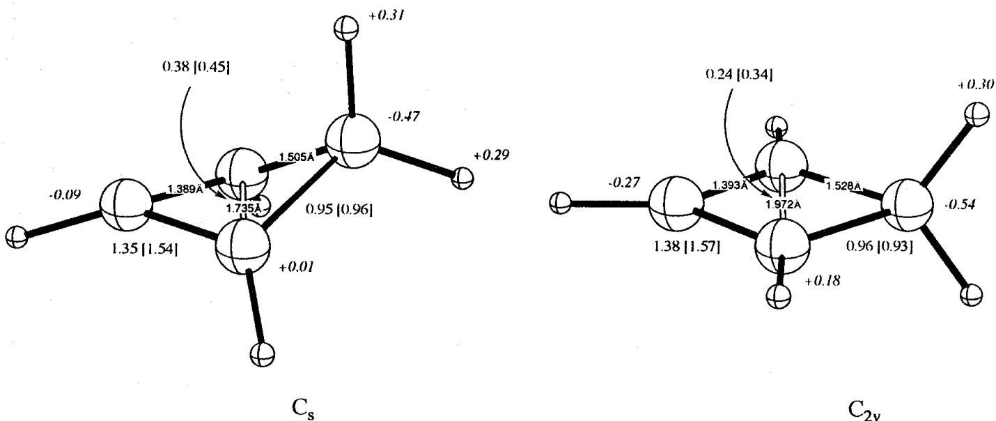
Figure 4. MP2 total response electron densities [for MP4(SDQ)/6-31G* geometries given in square brackets], NPA bond orders (Wiberg bond index) and NPA charges for the homocyclopropenylium ion at MP2(full)/6-31G**/MP2(full)/6-31G**
