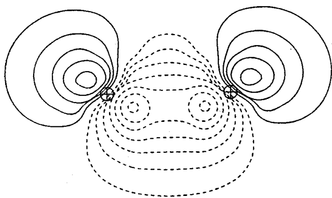
Figure 5. Contour plot of the 1,3-bonding orbital (NLMO) for the homotropylium ion at MP2(full)/6-31G*//MP2(full)/6-31G* in a plane perpendicular to the C 1 C 2 C 6 C 7 plane
