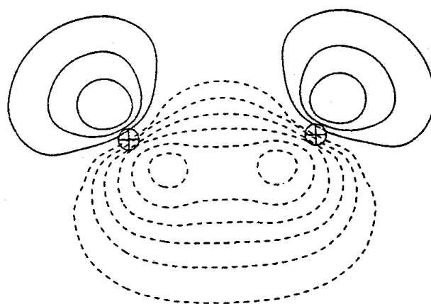
Figure 8. Contour plot of the 1,3-bonding orbital (NLMO) for the homodiborirane ion at HF/6-31G*//MP2(full)/6-31G* in a plane perpendicular to the B 1 C 2 B 3 plane
