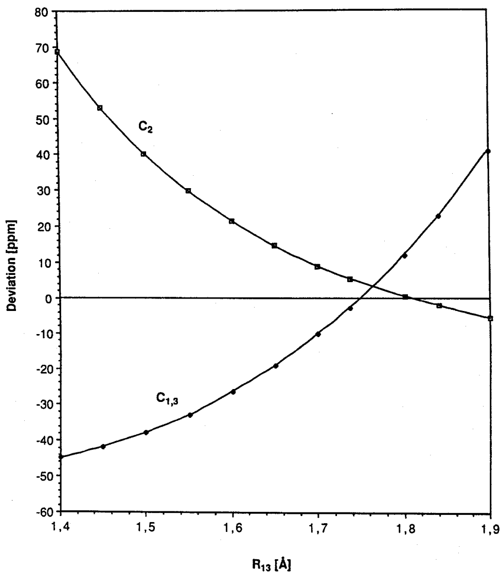
Figure 2. Differences between experimental and computed ^{13}\text{C} chemical shifts of the homocyclopropenylum cation as a function of the bond length C-1—C-3. Geometries are optimized at the MP2(full)/6-31G* level with fixed C-1—C-3 bond length. Chemical shifts are computed using the 6-31G** standard basis set
