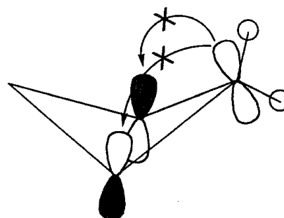
LUMO (allyl) - pseudo- \pi ( \text{CH}_2 ) interaction
