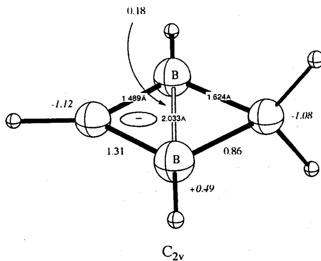
Figure 7. NPA bond orders (Wiberg bond index) and NPA charges for the homodiborirane ion at HF/6-31G*//MP2(full)/6-31G*
