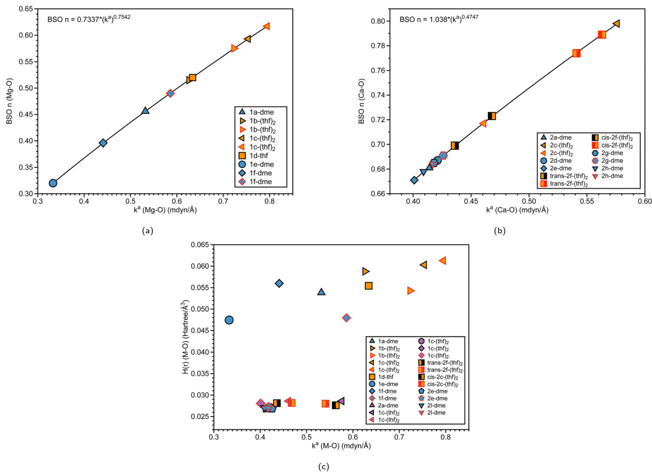
Fig. 7 (a) BSO n (Mg–O) vs. local force constant k^a (Mg–O) (mdyn/Å). (b) BSO n (Ca–O) vs. local force constant k^a (Ca–O) (mdyn/Å). The black outline represents O_a , while the red outline represents O_b (see Fig. 1 and Fig. 2). (c) Energy density H(r) (Hartree/Å 3 ) vs. local force constant k^a (M–O) (where M = Mg, Ca). The black outline represents O_a , while the red outline represents O_b at the B3LYP-D3/def2-TZVP level of theory.
